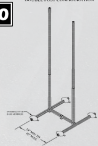
TTSK175-2 DOUBLE POST CONFIGURATION
